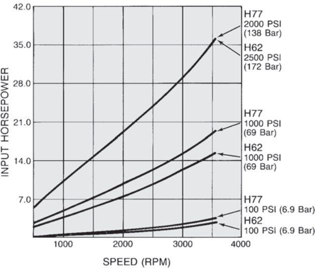
H62/H77 Horsepower/Speed
