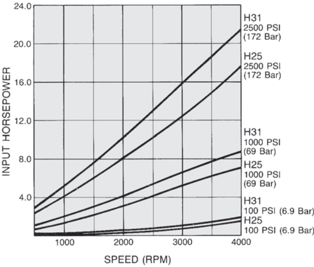
H25/H31 Horsepower/Speed
