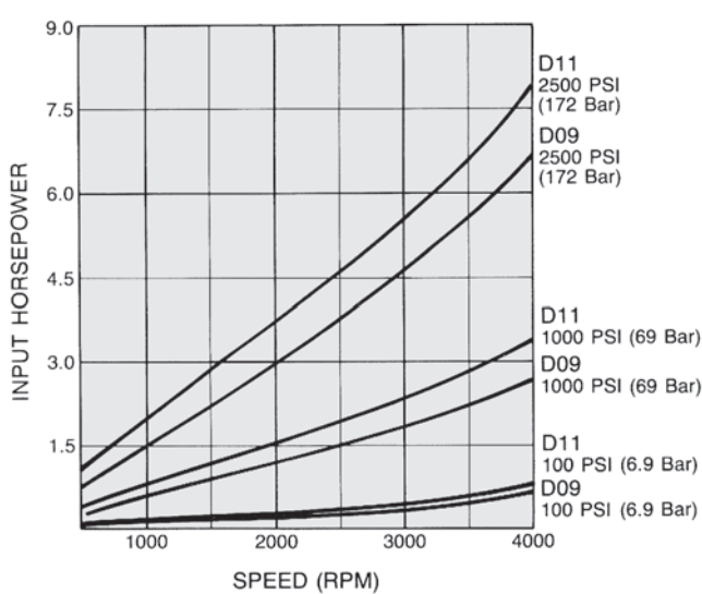
D09/D11 Horsepower/Speed
