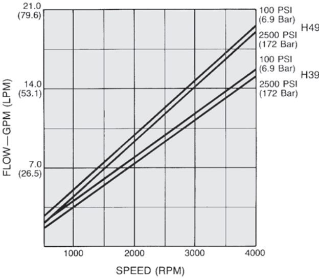
H39/H49 Flow/Speed
