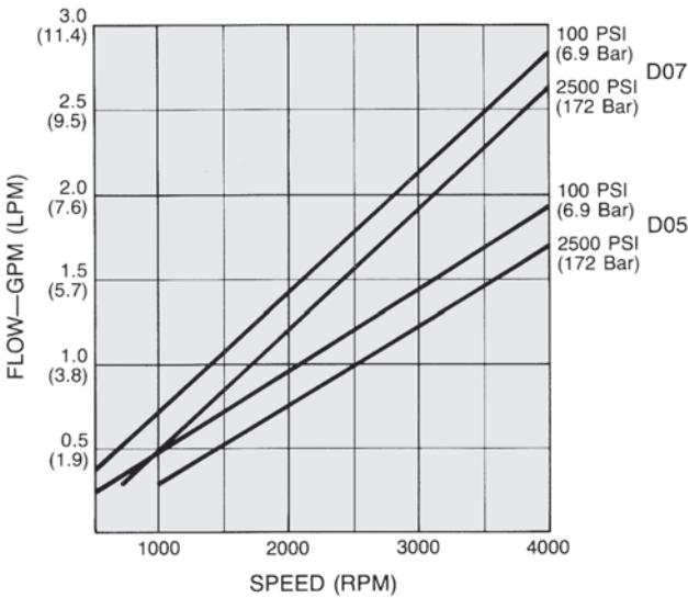
D05/D07 Flow/Speed
