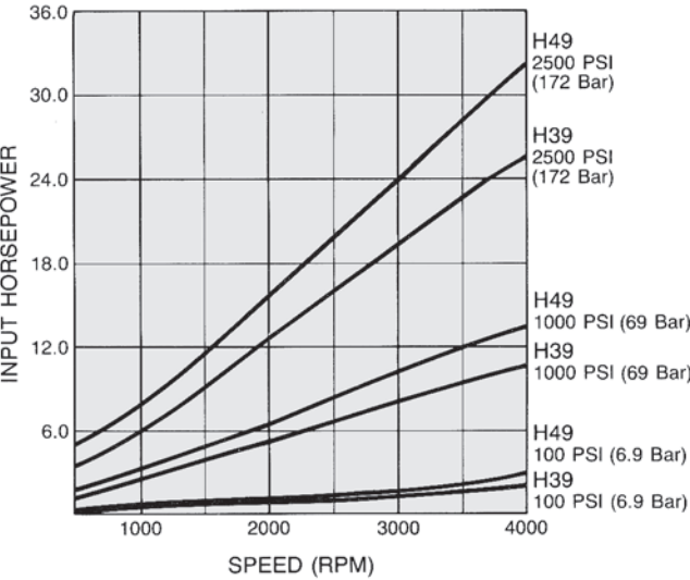
H39/H49 Horsepower/Speed
