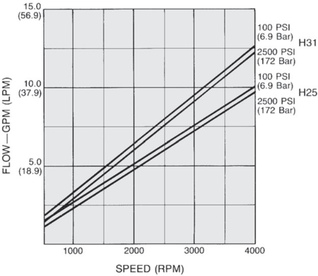
H25/H31 Flow/Speed
