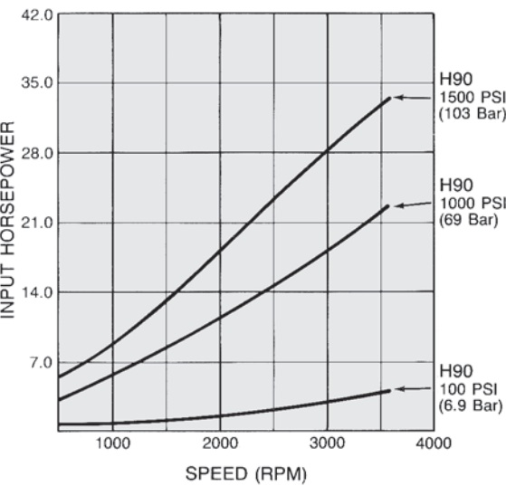
H90 Horsepower/Speed
