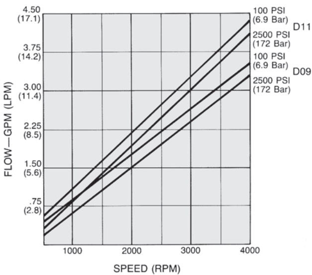
D09/D11 Flow/Speed
