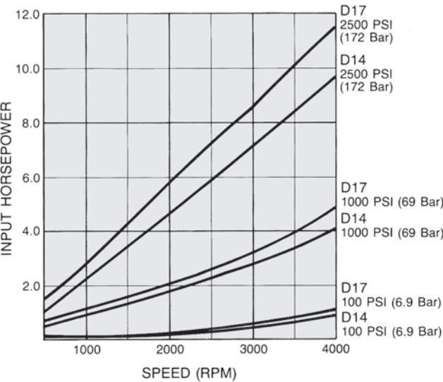
D14/D17 Horsepower/Speed
