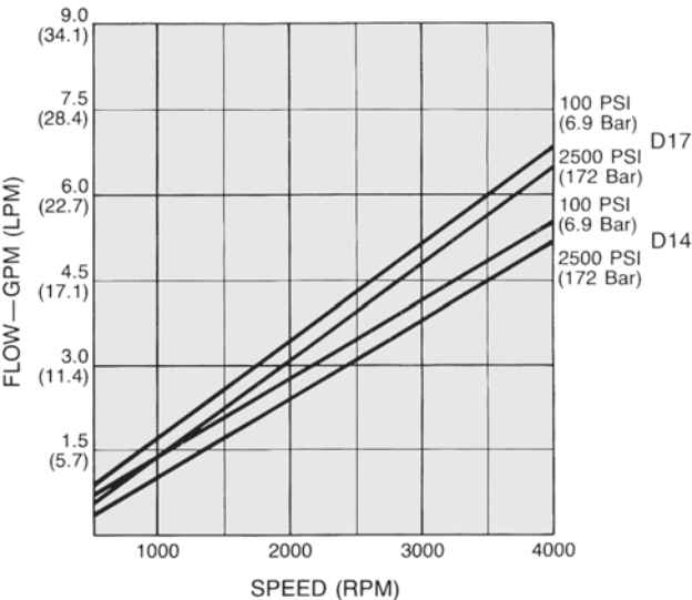
D14/D17 Flow/Speed
