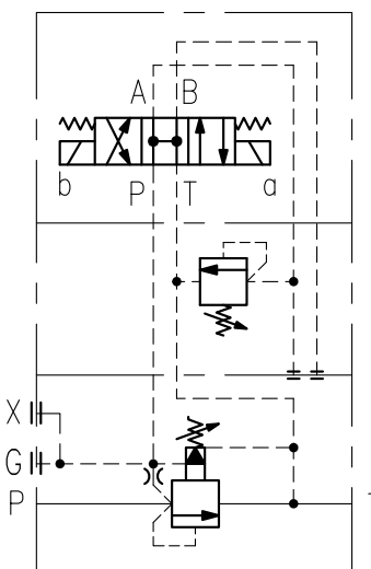
Pressure Relief, 2 pressure + unloading, normally unloading, energize A solenoid for low pressure, energize B solenoid for high pressure
