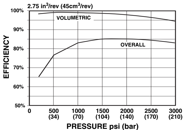
EFFICIENCY @ 1200 rpm
