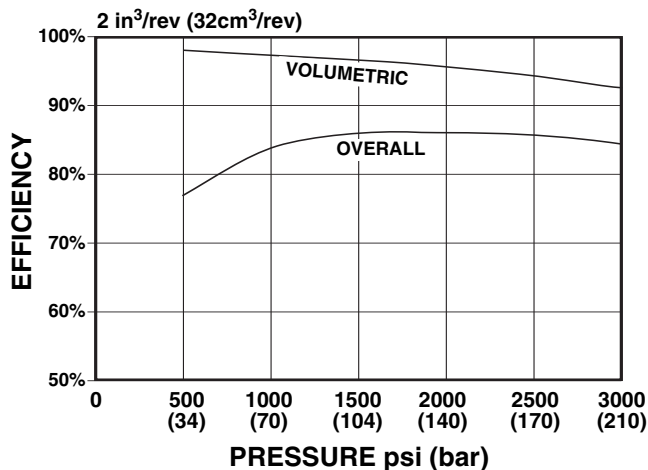
EFFICIENCY @ 1800 rpm
