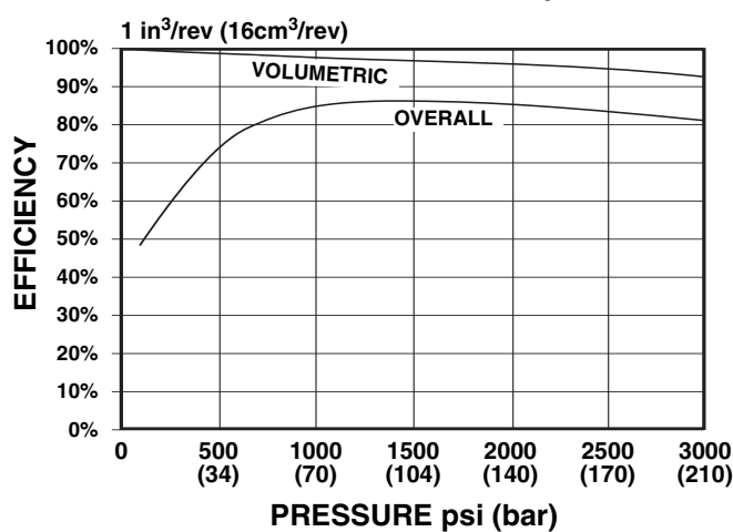
EFFICIENCY @ 1800 rpm
