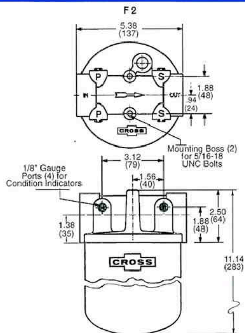
ELEMENT THREAD REFERENCE 1 1/2-16 UN-2B
