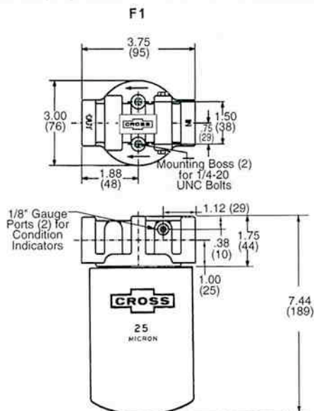
ELEMENT THREAD REFERENCE 1-12 UNF-2B
