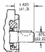
SHAFT C*
