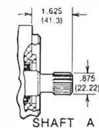
SHAFT A
