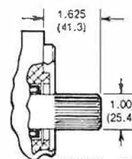
SHAFT B
