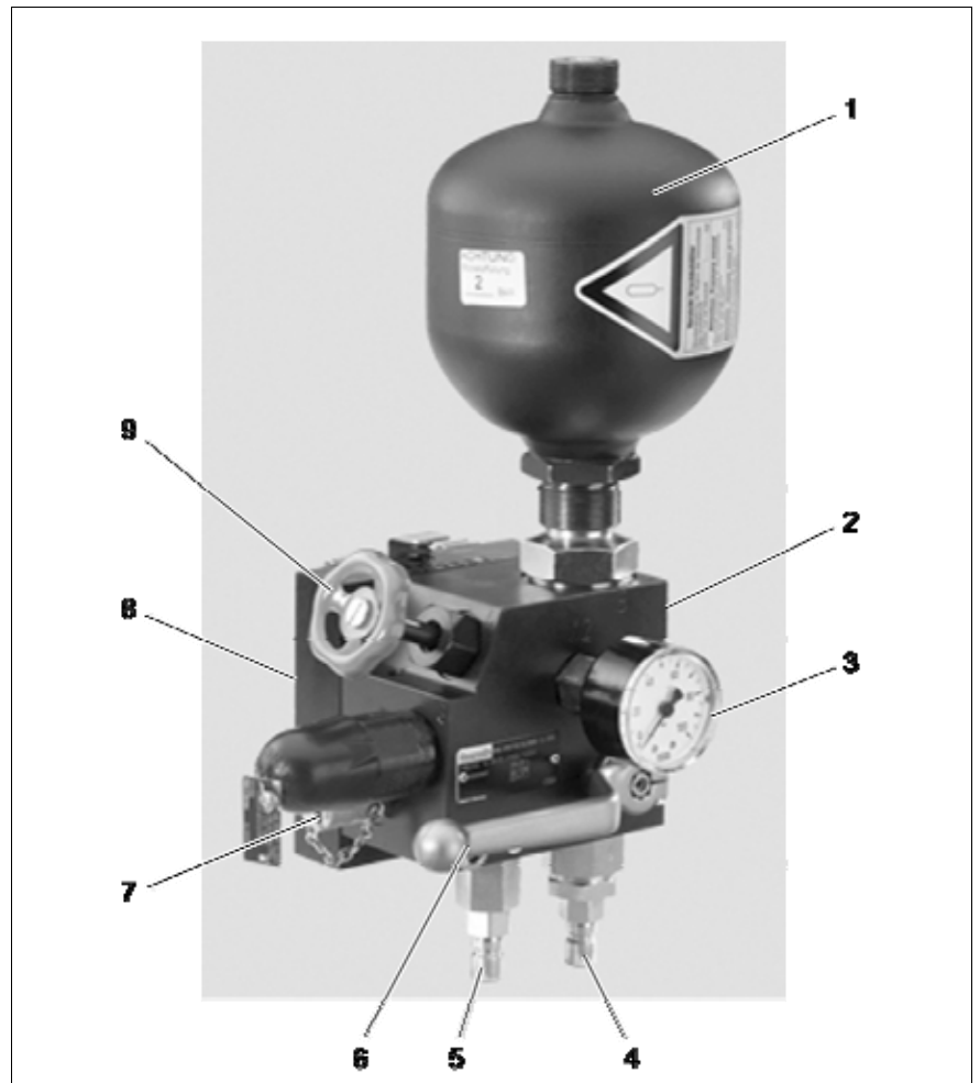
Fig. 3: Accumulator assembly DZ3.2 didactic hydraulic accumulator
