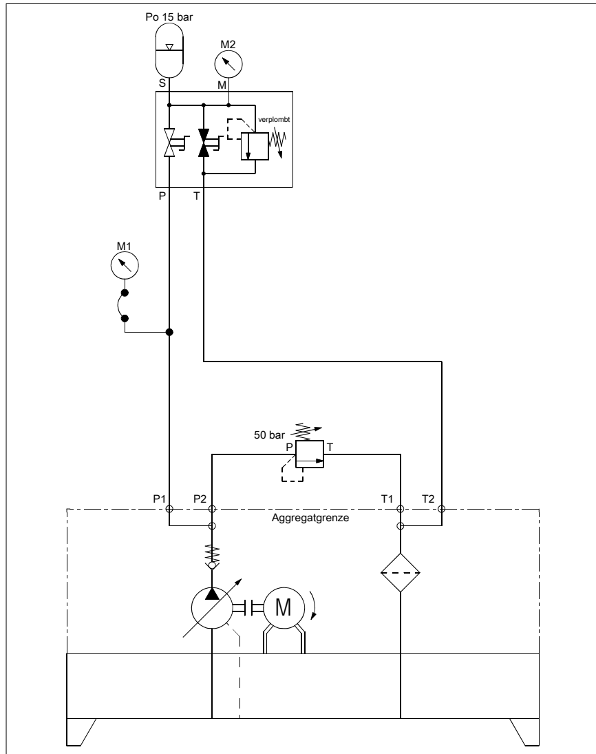
Fig. 6: Hydraulic diagram accumulator assembly DZ3.2 didactic hydraulic accumulator
