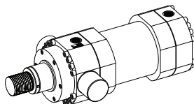
G (ISO MT1) = front trunnion mounting
