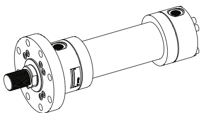
A (ISO MF3) = front round flange mounting
