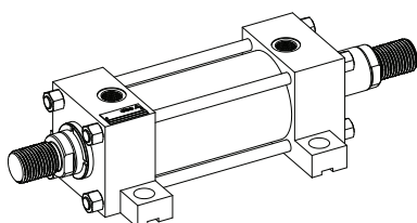
E = feet mounting for double rod
