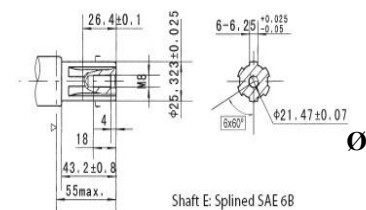
Shaft E: Splined SAE 6B
