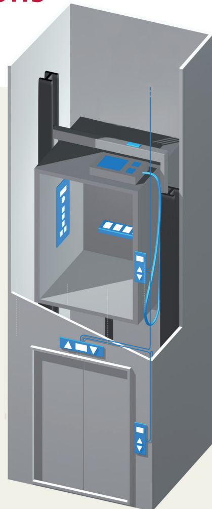
Shaft wiring and control panels for 2 or 3 stops
