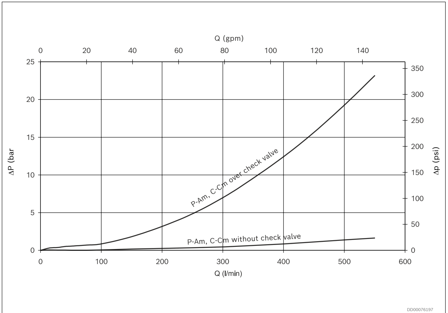
Fig. 9: Pressure loss P-Am, C-Cm over check valve, and without check valve. VCBCA 480 Viscosity 40 cSt
