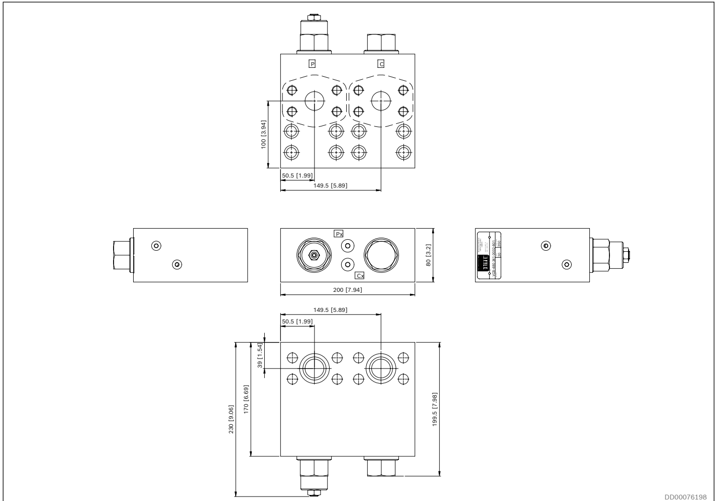
Fig. 10: Dimensions VCBCA 480 configuration B
