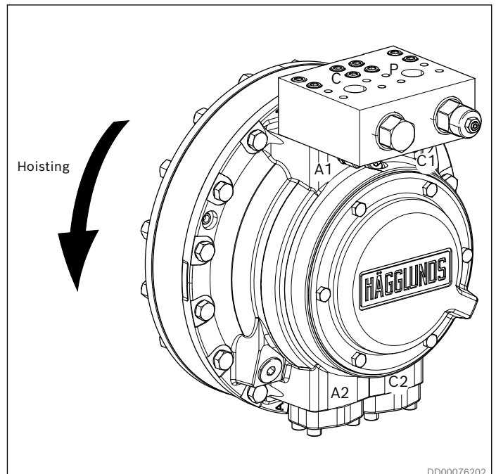
Fig. 13: Example CA configuration C: High pressure in P valve / C1 motor (Hoisting), motor shaft rotating clockwise viewed from the motor shaft side. Lowering in C valve / A1 motor port
