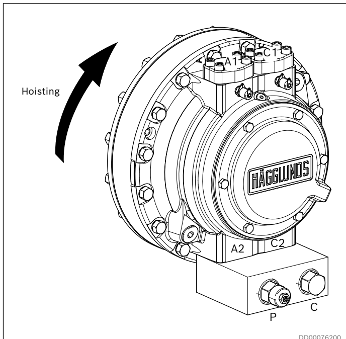
Fig. 12: Example CA configuration C: High pressure in P valve / A2 motor (Hoisting), motor shaft rotating counter clockwise viewed from the motor shaft side. Lowering in C valve / C2 motor port
