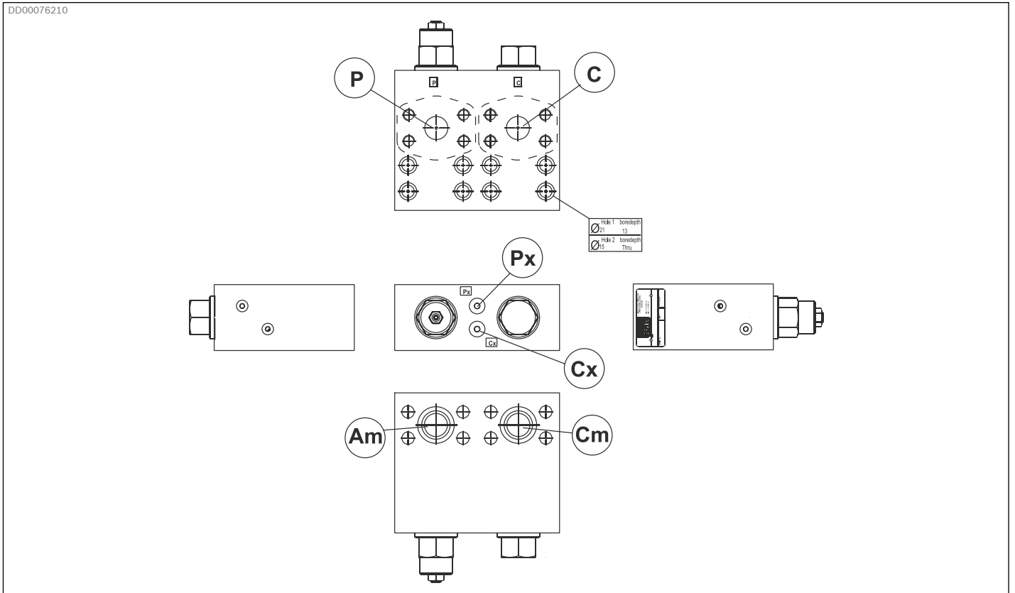
Fig. 17: Installation drawing VCBCA 480
