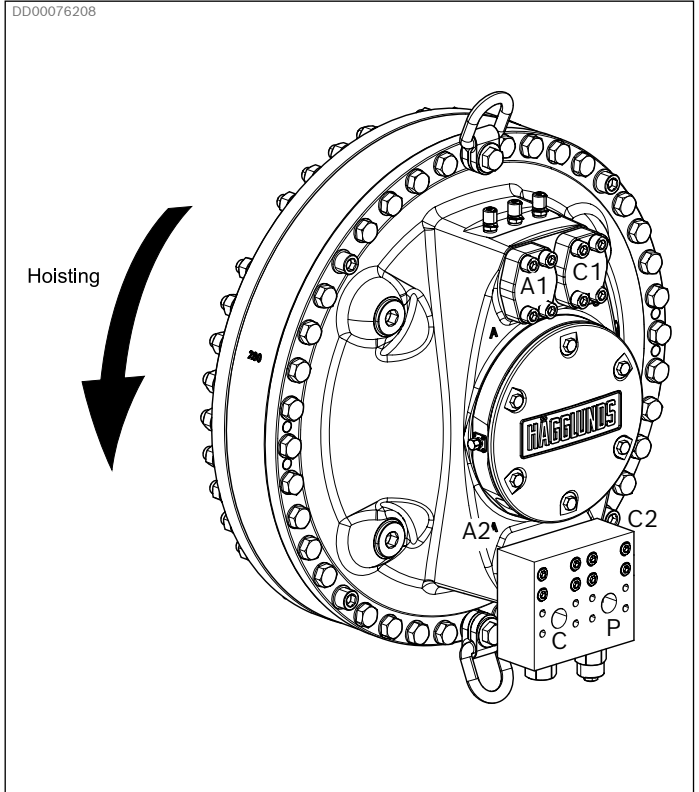
Fig. 16: Example CB configuration C: High pressure in P valve / C2 motor (Hoisting), motor shaft rotating clockwise viewed from the motor shaft side. Lowering in C valve / A2 motor port
