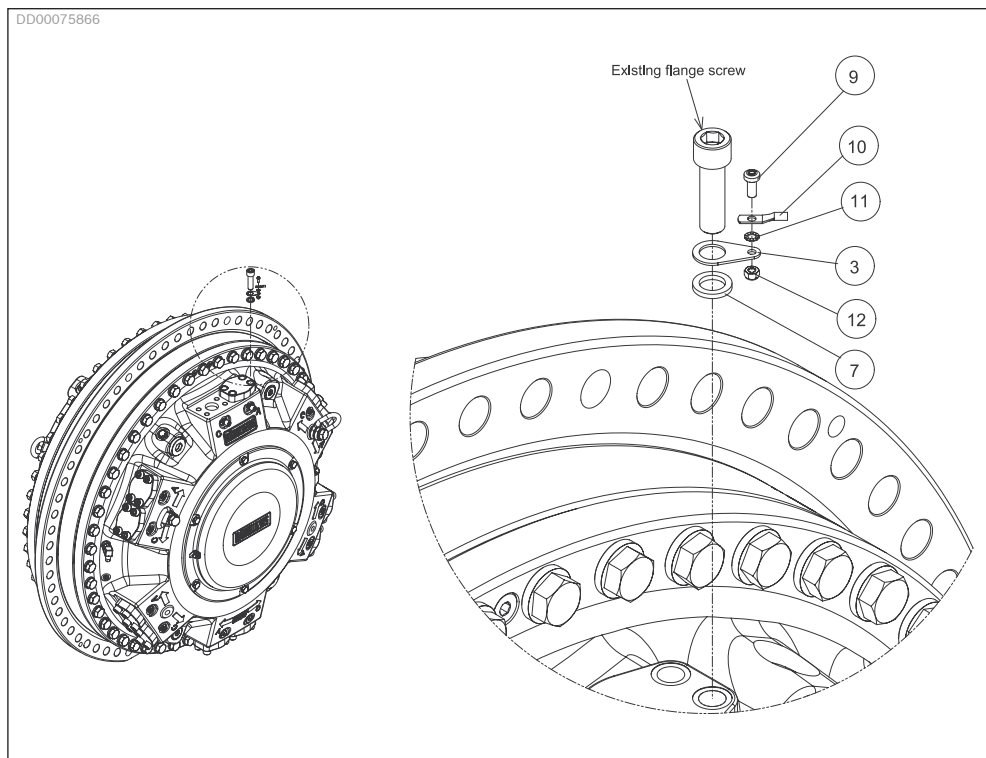
Fig. 7: Grounding point example, Hägglunds CBM
