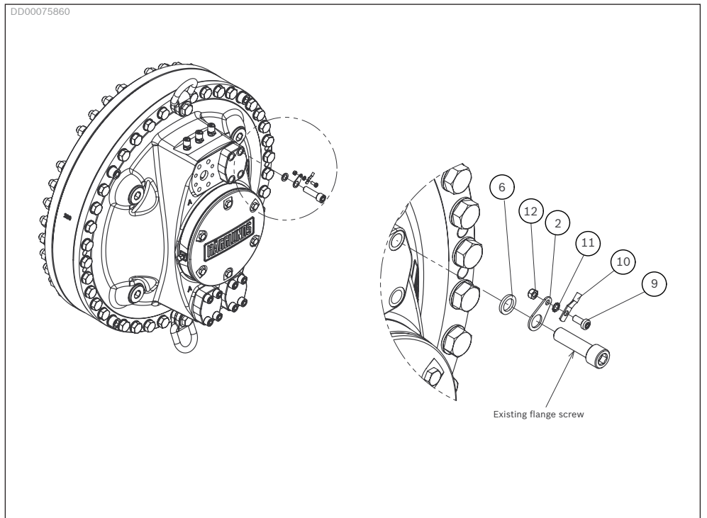
Fig. 5: Grounding point example, Häglunds CB
