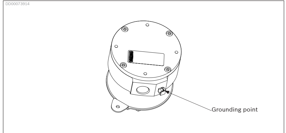
Fig. 10: Grounding of SPDB2
