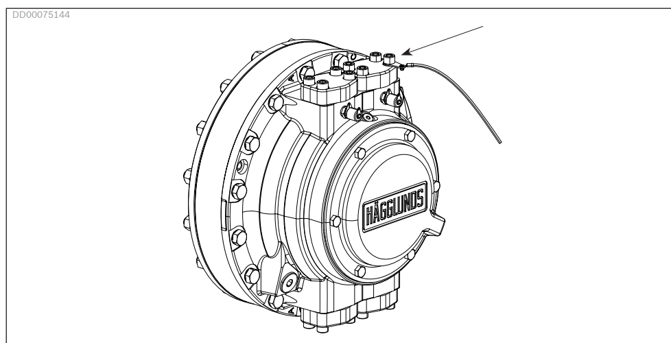
Fig. 3: Grounding of motor
