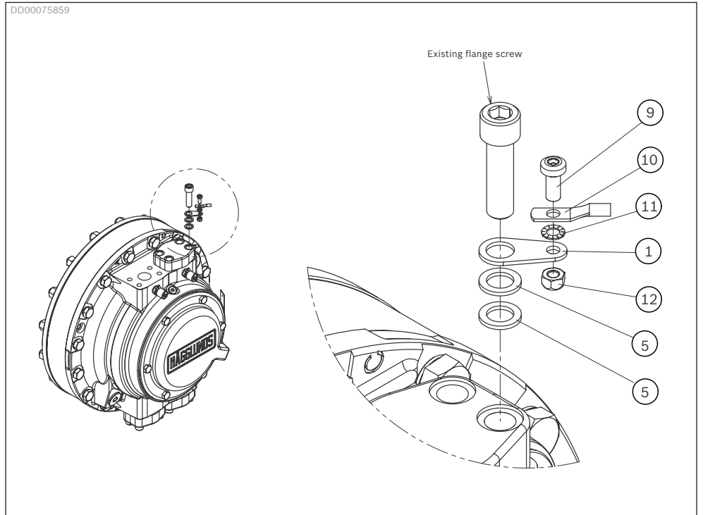
Fig. 4: Grounding point example, Häglunds CA
