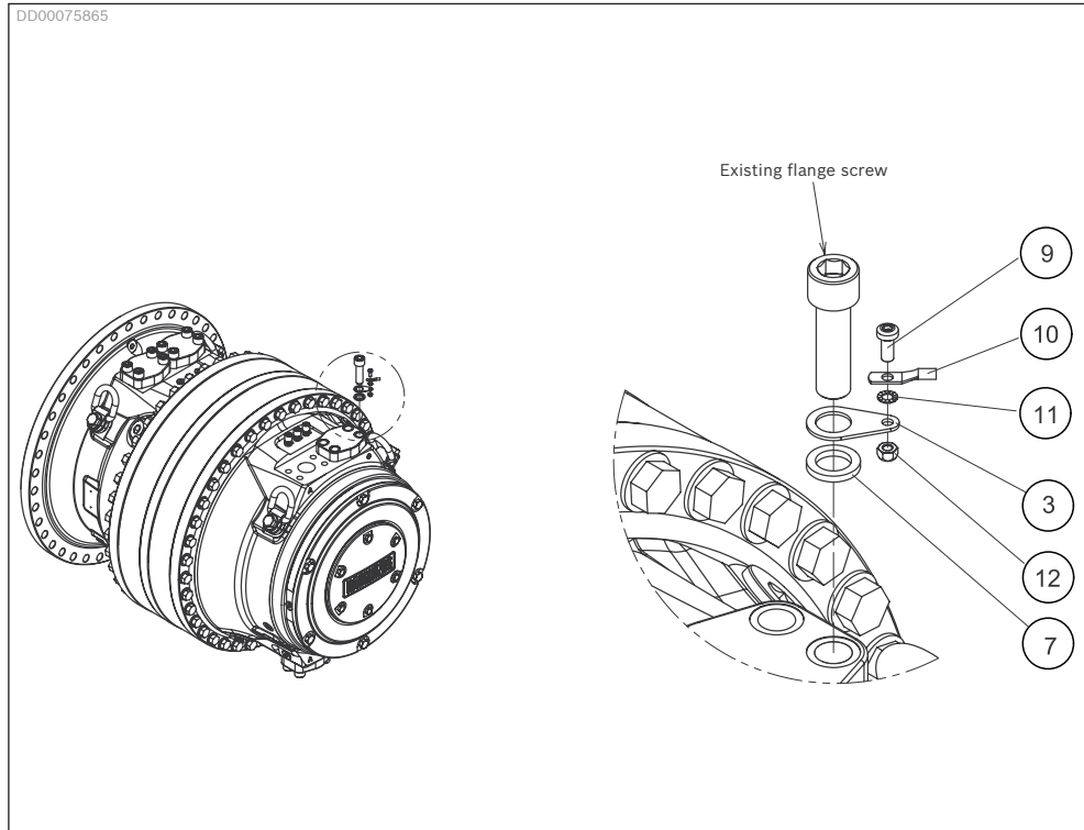
Fig. 6: Grounding point example, Hägglunds CBP
