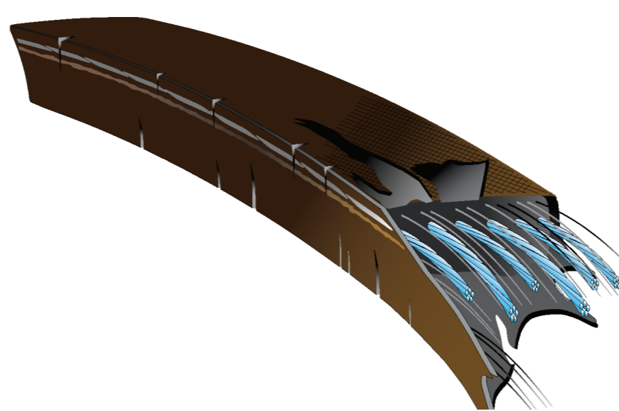
18. BROKEN BELT
