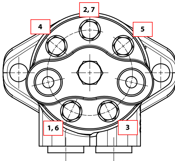
Figure 14: Tightening sequence
