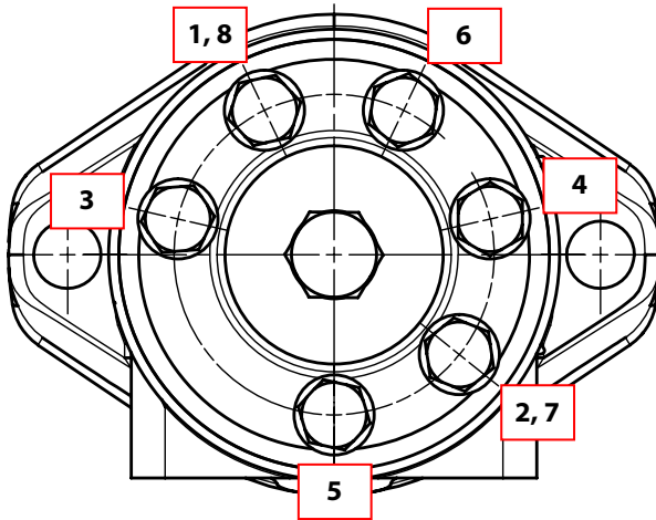
Figure 13: Tightening sequence
