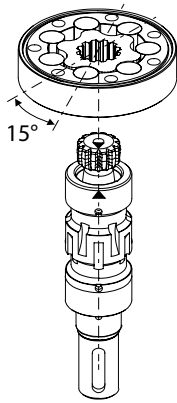
Figure 11: Installation of gearwheel to cardan shaft
