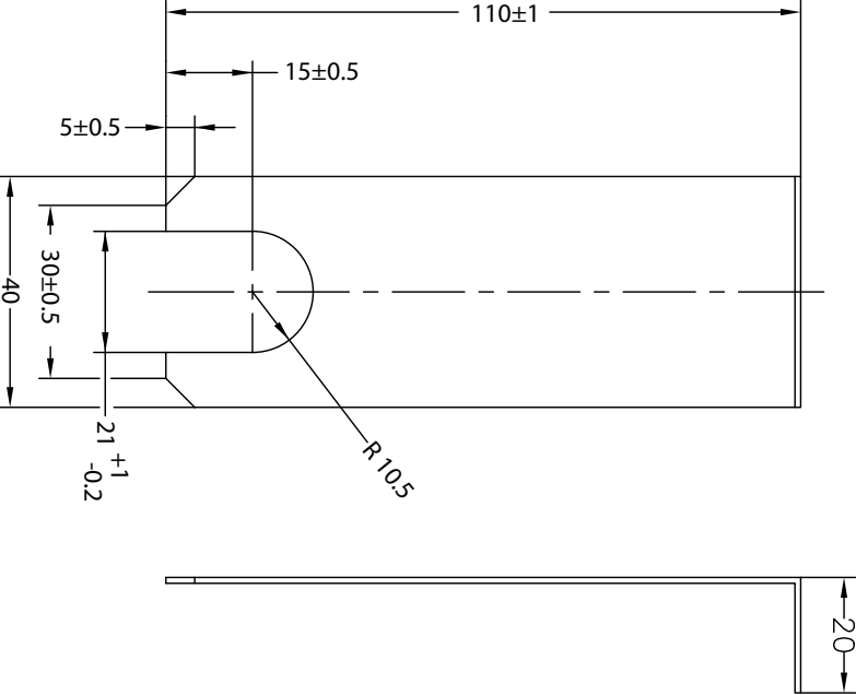
Figure 33: Fork
