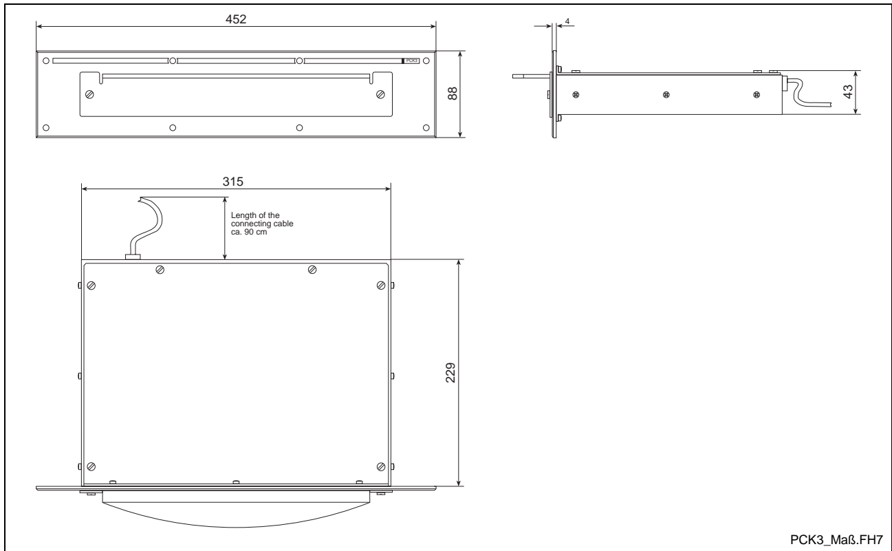
Figure 5-1: Enclosure dimensions
