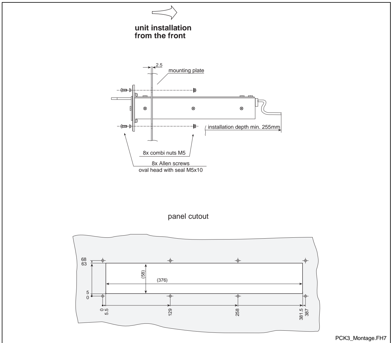
Figure 5-2: Mounting dimensions
