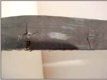
Figure 19 - Tensile cord failure from debris
