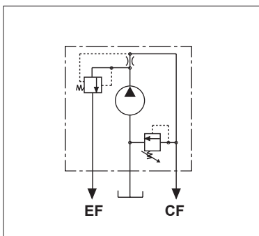
CF= Priority flow port EF= Excess flow port
