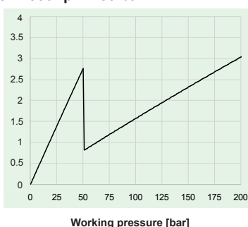
Example: 6.5cc/16cc - 1500 rpm - 50 bar
