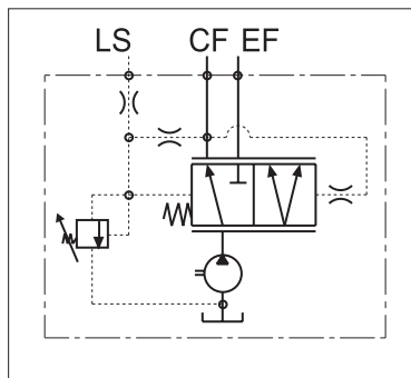
CF= Priority flow port EF= Excess flow port LS= Load sensing signal port
