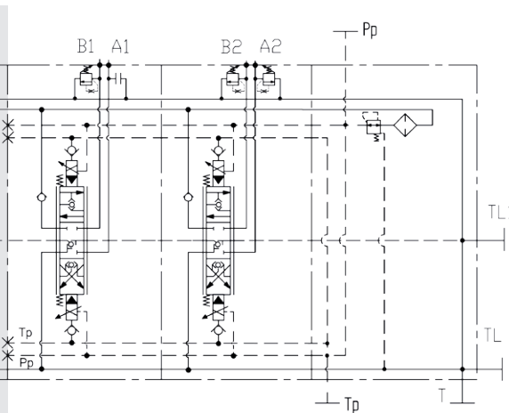
Example of hydraulic circuit
