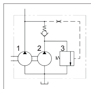
1= Stage high pressure 2= Stage low pressure 3= Unloading valve
