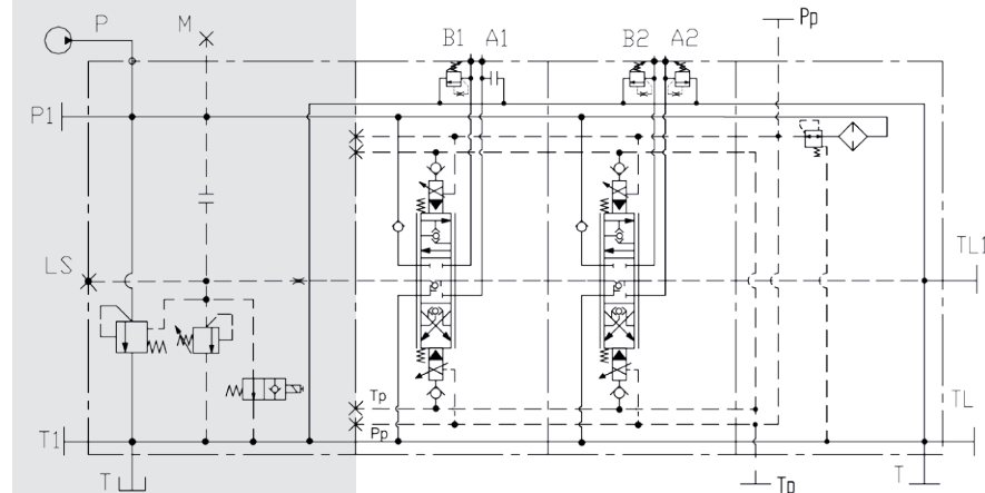
Inlet section for fixed displacement pumps
