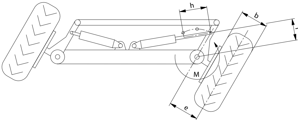
Figure 7: Steering geometry
