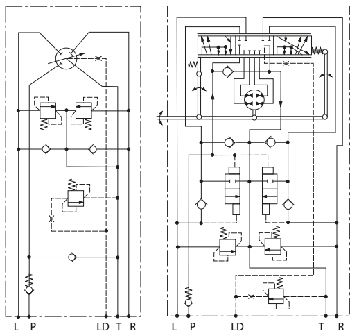
Figure 5: LAGU LDA / NR schematic
