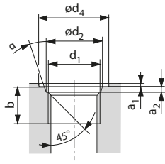
Figure 19: UNF, metric thread
