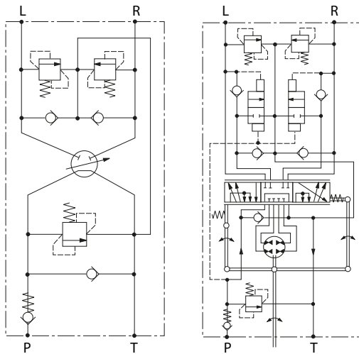
Figure 2: LAGU OC / NR schematic
