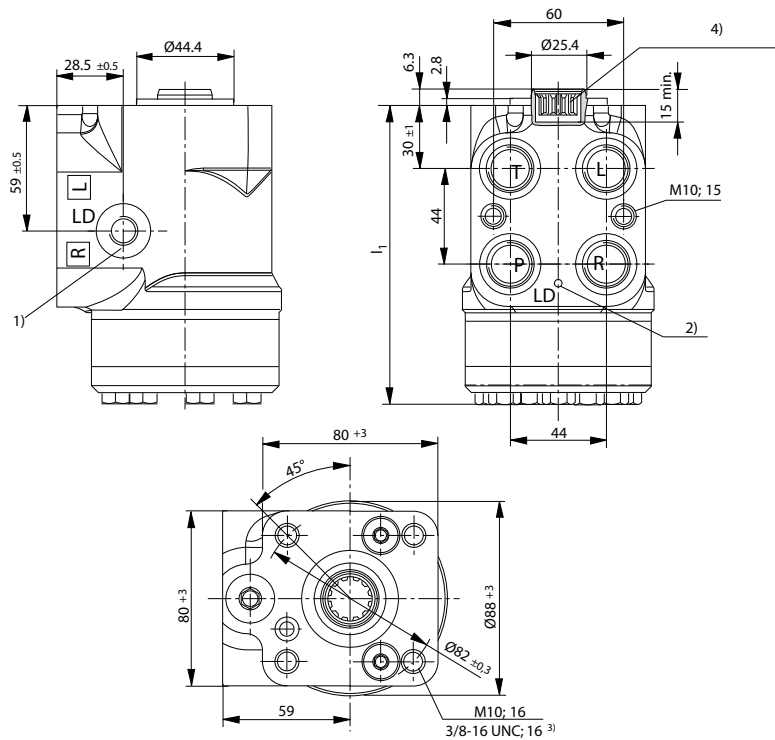
Figure 17: Dimensions for LAGU and LAGU LD & LDA versions (in mm)
