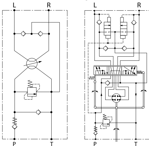
Figure 3: LAGU OC / R schematic
