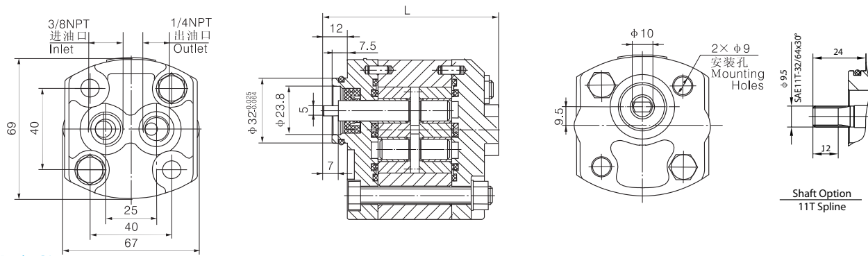
CBK-F*DF Outline Dimension (Rear in/rear out)
