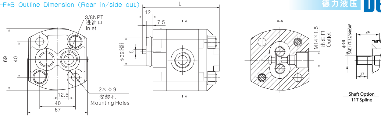
CBK-F*CF Outline Dimension (Side in/side out)
