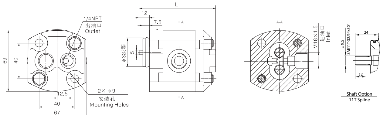
CBK-F*AF Outline Dimension (Side in/rear out)
