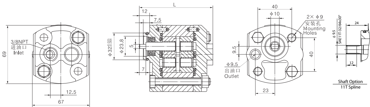
CBK-F*AF Outline Dimension (Side in/rear out)
