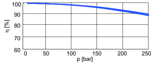
Volumetric efficiency
