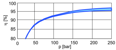
Hydromechanical efficiency
