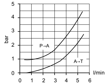
Plug 00VRP00
