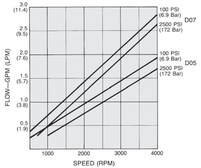
D05/D07 Flow/Speed
