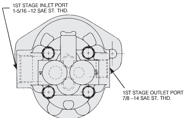
Rear (CCW) View
