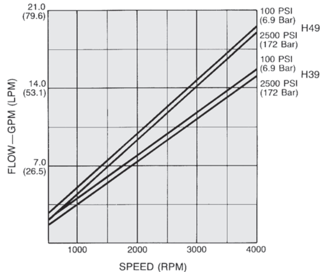
H39/H49 Flow/Speed
