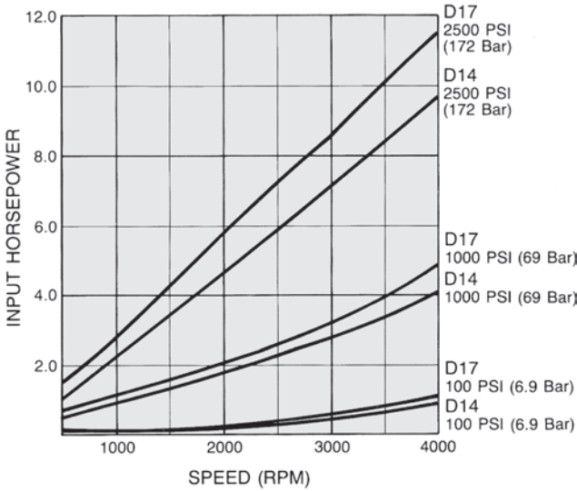
D14/D17 Horsepower/Speed
