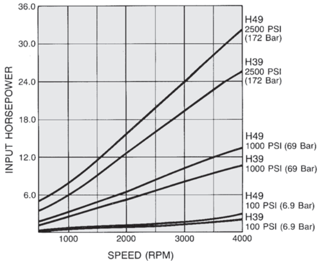
H39/H49 Horsepower/Speed
