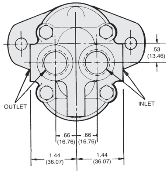
Rear View
