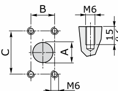
F: SAE J518-1 connection
