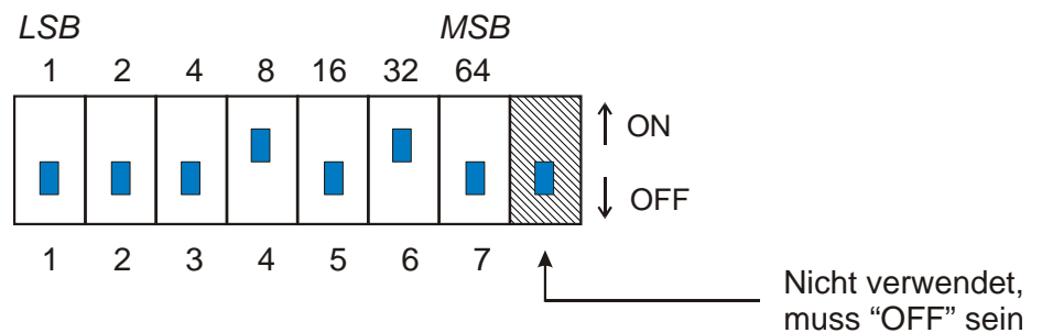
Fig. 1 Address dipswitches
