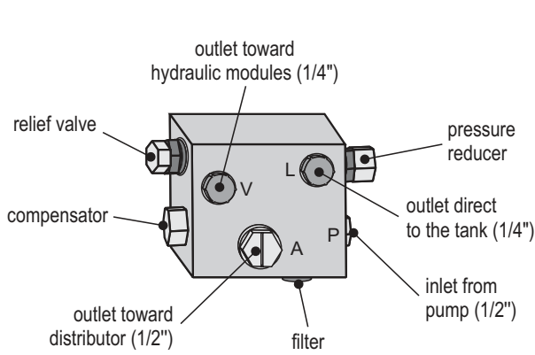
A5000020011 - Max flow = 70 l/min
