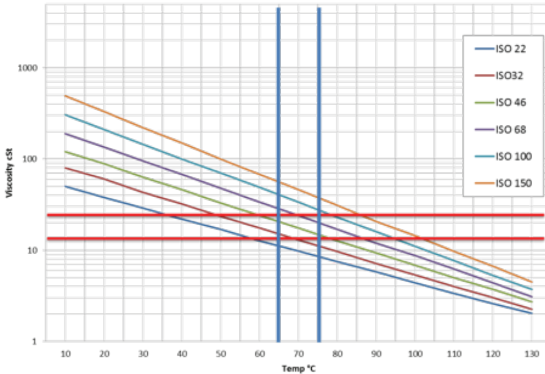
Figure 2: Viscosity-temperature profile for mineral oils with a viscosity index of 95 showing the optimum viscosity grade to maintain adequate oil film thickness at operating temperatures
