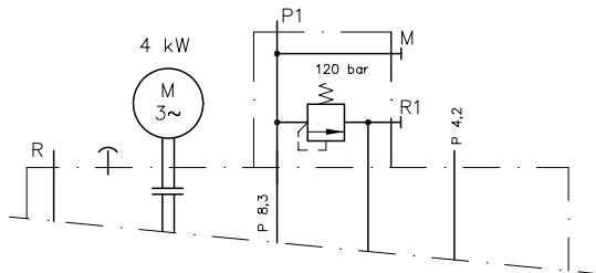
Pressure port 1 safeguarded on the power pack
