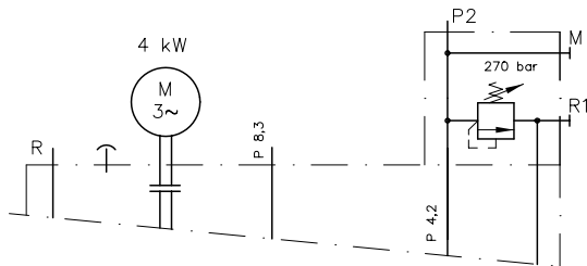
Pressure port 2 safeguarded on the power pack
