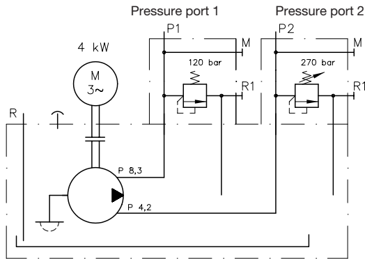
Pressure ports 1 and 2 safeguarded on the power pack
