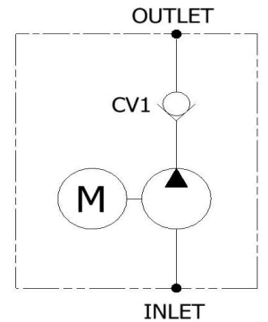
HYDRAULIC SCHEMATIC
