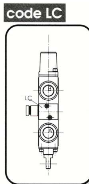
Working section with compensated flow limiting valve
