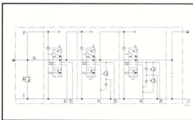
Series circuit
