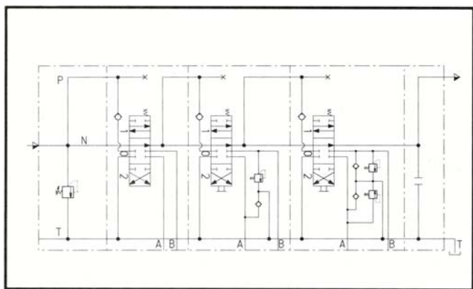
Tandem circuit
