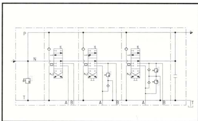
Parallel circuit
