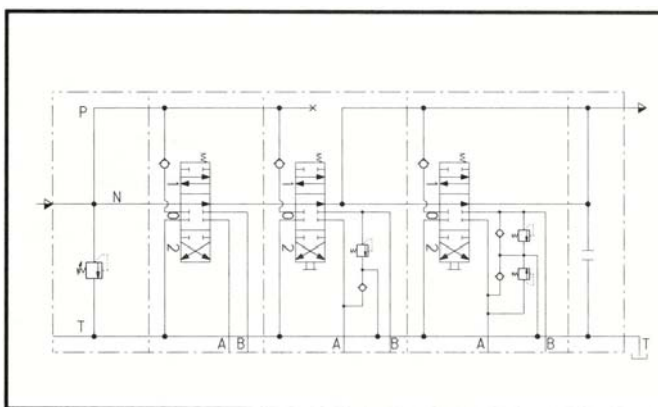
Mixed circuit
