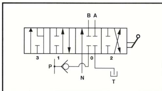
Double acting spool with float spool position (spool out)
