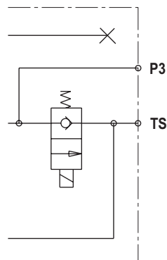
Normally closed
