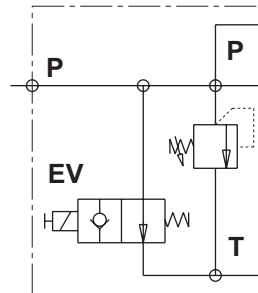
Normally opened
