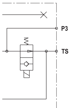
Normally opened
