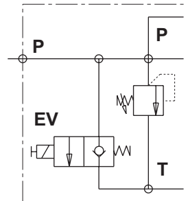
Normally closed
